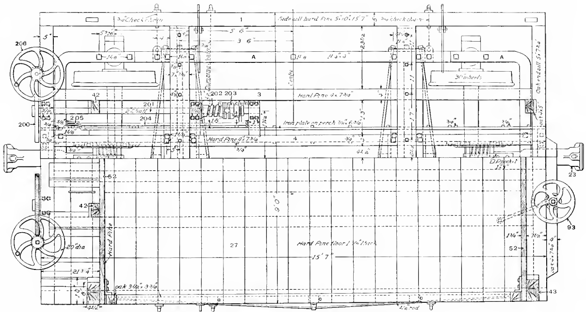
Fig. 337. Plan showing Floor and Underframe.
